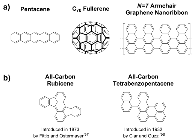
Figure 1. a) Typical carbon-based materials, including pentacene (left), C 70 fullerene (middle), and an N=7 armchair graphene nanoribbon (right). b) The classic all-carbon rubicene and tetrabenzopentacene molecules.
